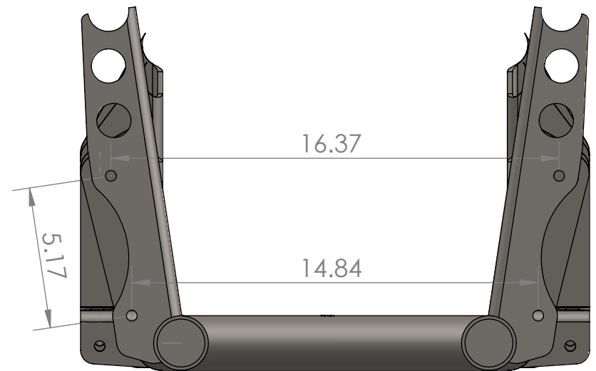
REAR VIEW
